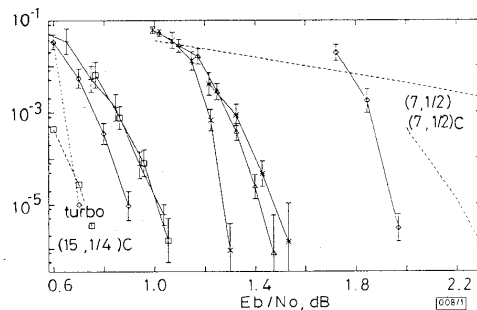
Fig. 1 GL codes' performance over Gaussian channel compared with that of standard textbook codes and state of the art codes — Gaussian channel, - - - (right) standard textbook, . . . (left) state of the art
