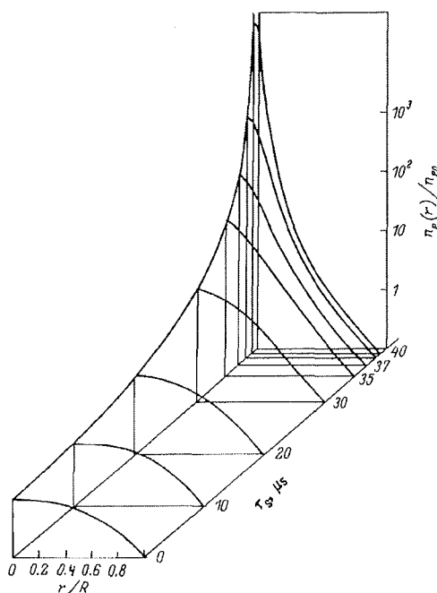
FIG. 5. Radial distribution n_e(r) as a function of time for A > 0 in an argon discharge. p = 11.4 torr, n_{e0} = 10^{10} cm ^{-3} , \tau_s = 39 \mu s.
