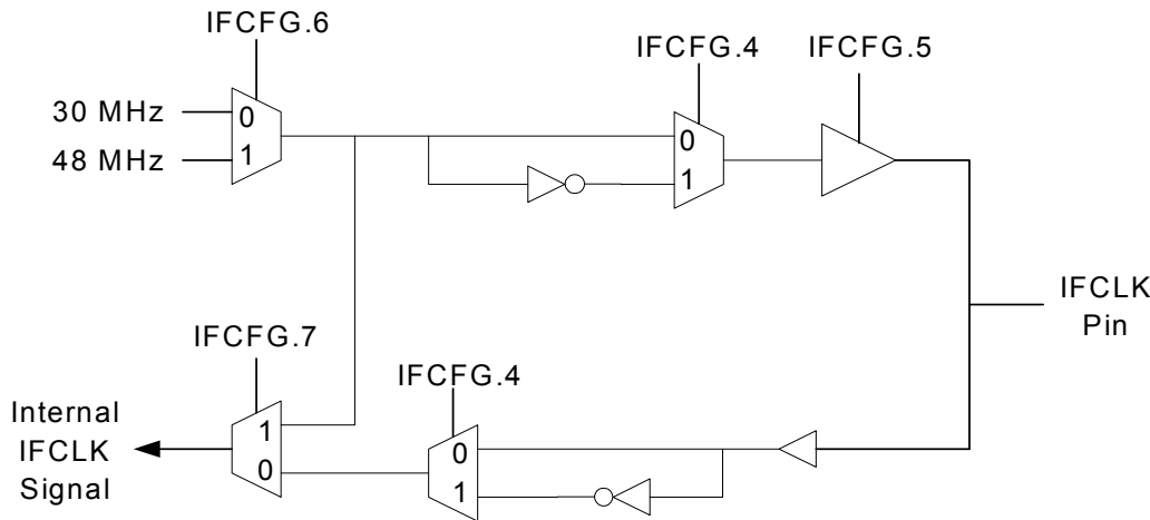
Figure 9-6. IFCLK Configuration
