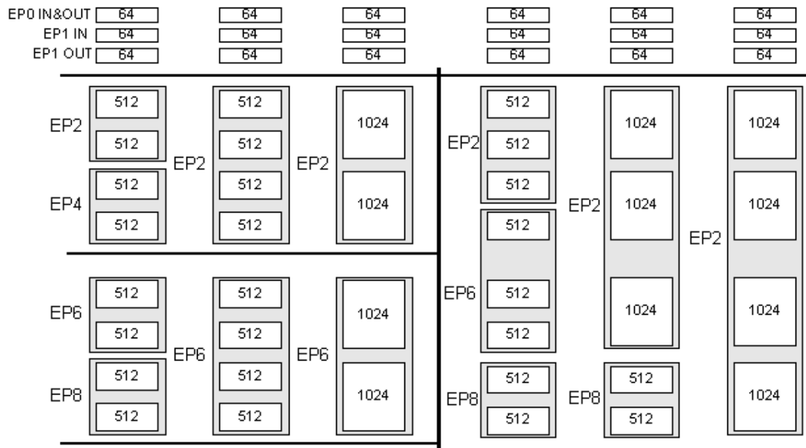
Figure 1-15. FX2 Endpoint Buffers
