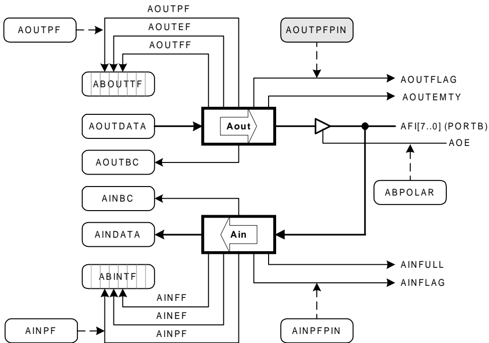
Figure 7-30. AOUTFPIN's Role in the FIFO A Register
