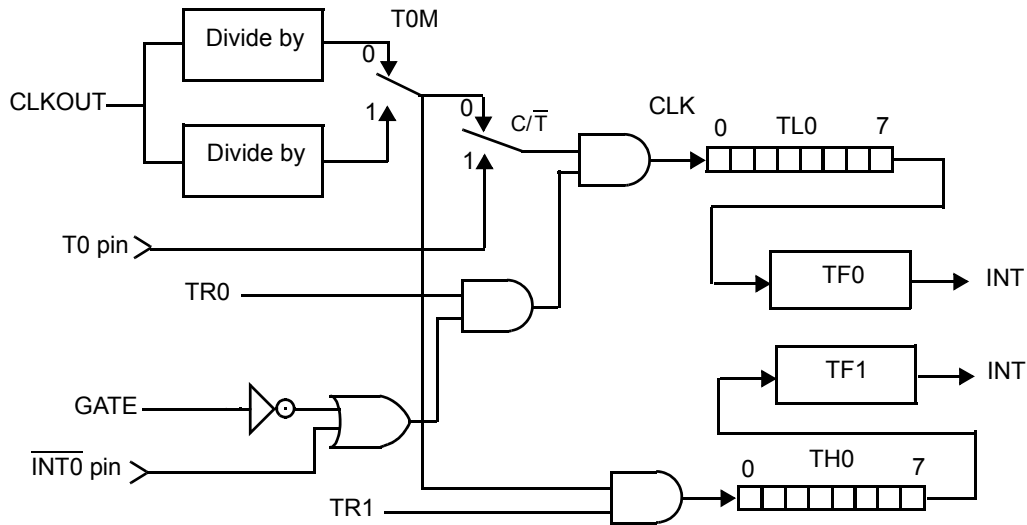
Figure 14-3. Timer 0 - Mode 3
