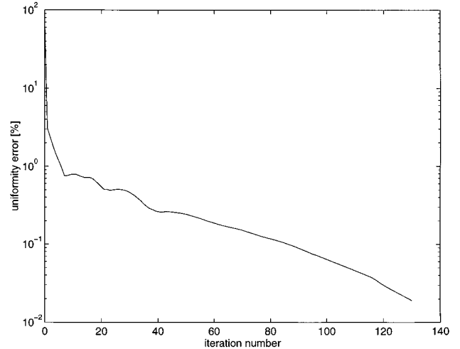
Fig. 5. Uniformity error versus the number of iterations for the design of the near near-field kinoform.
