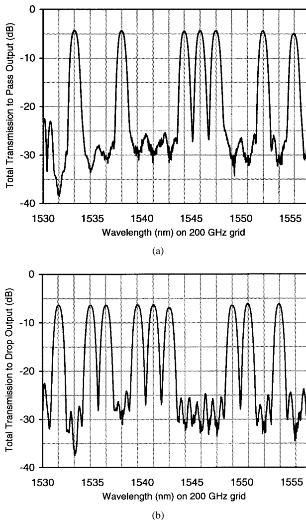
Fig. 6. (a) PASS and (b) DROP transmission of ASE input dropping eight of 16 channels.
