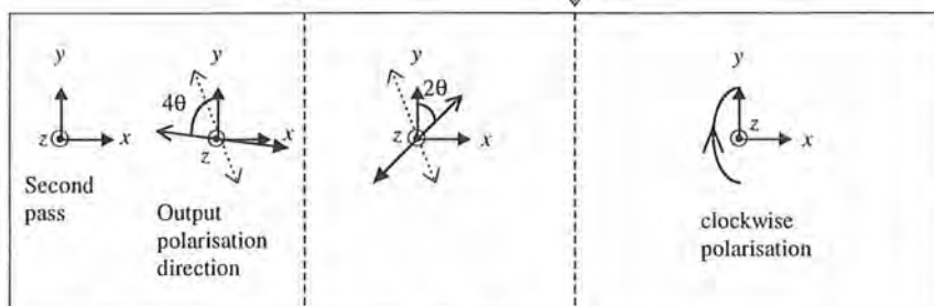
Polarisation diagrams of the reverse pass
