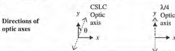
Polarisation diagrams of the forward pass
