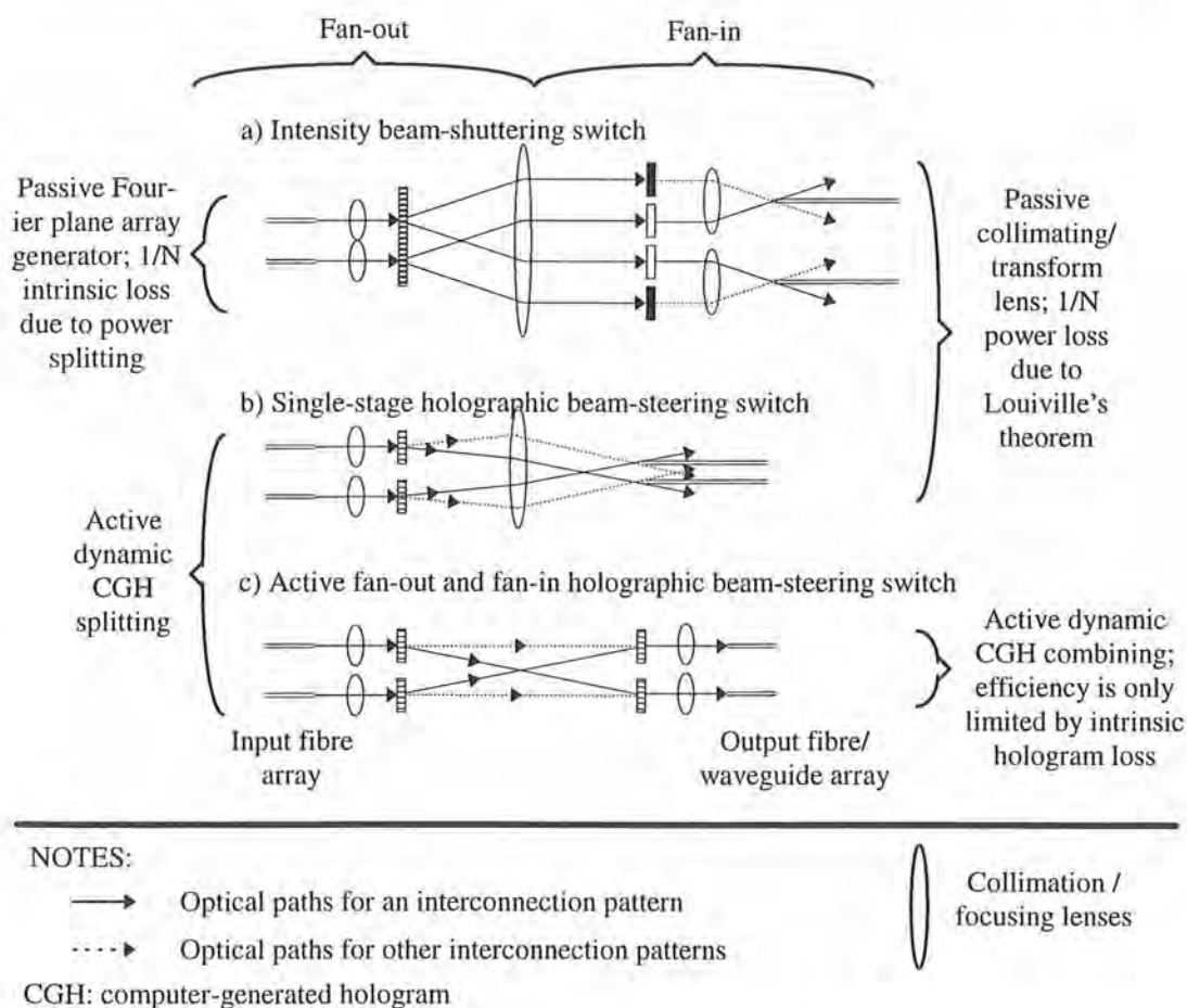
Figure 2.5: Single-mode fibre to fibre free-space switch techniques.
