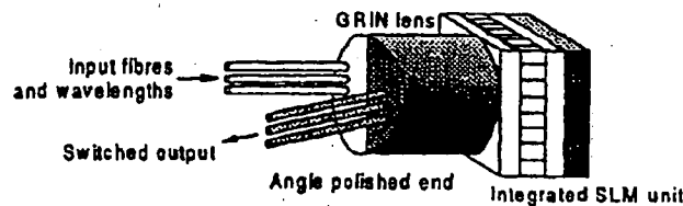
Figure 8: Packaged, integrated space-λ switch
