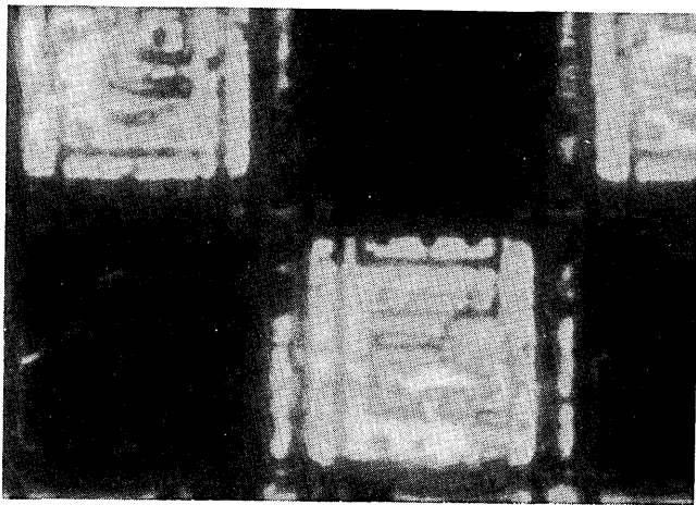
Fig. 3. Higher-magnification microphotograph of the square array showing structure within the elements due to the underlying circuitry topography.
