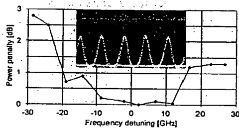
Fig. 6. Power penalty induced by filter shape as a function of detuning the optical carrier frequency. Inset: eye diagram at zero offset.
