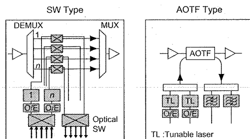
Figure 1 SW and AOTF types of OADM architectures.
