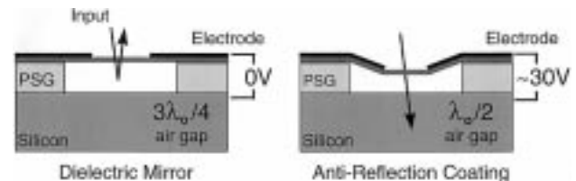
Fig. 1. MARS micromechanical modulator concept.
