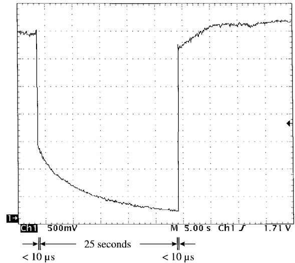
Fig. 4. Dynamic attenuation response to 60-V square-wave drive.
