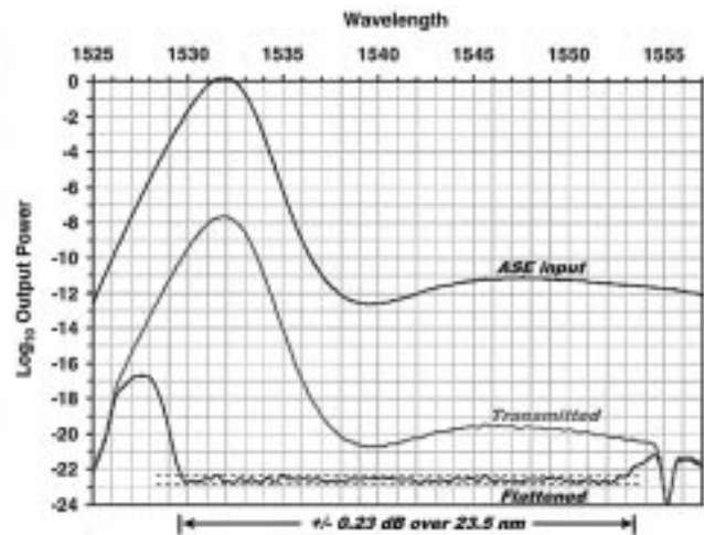
Fig. 5. Equalized erbium-doped fiber amplifier ASE.
