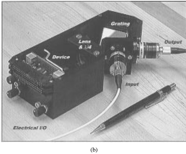
Fig. 2. (a) Optical design. (b) Optomechanical WDM package.
