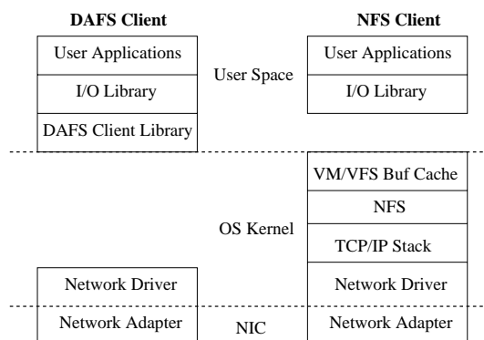
Figure 1: User-level vs. kernel-based client file system structure.
