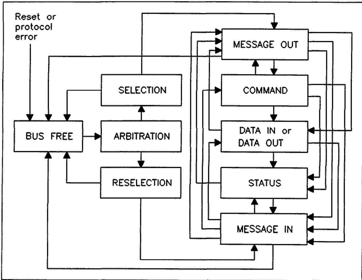
Figure 16 - Phase sequences
