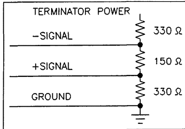
Figure 11 - Termination for differential device
