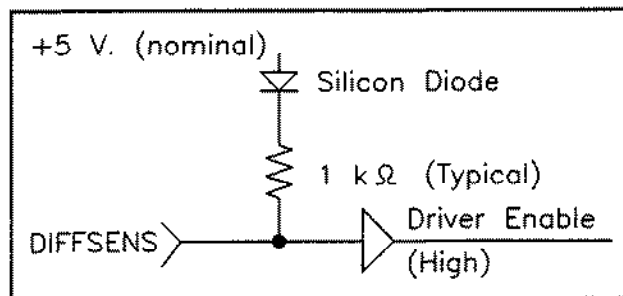
Figure 11 - Termination for differential device
