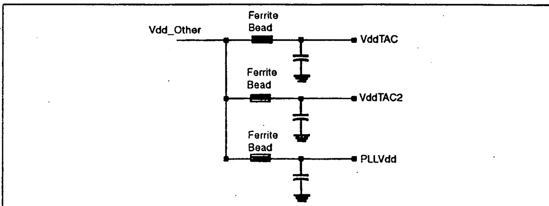
Figure A.1.7 Multiple Ferrite Beads for Maximum Isolation Method
