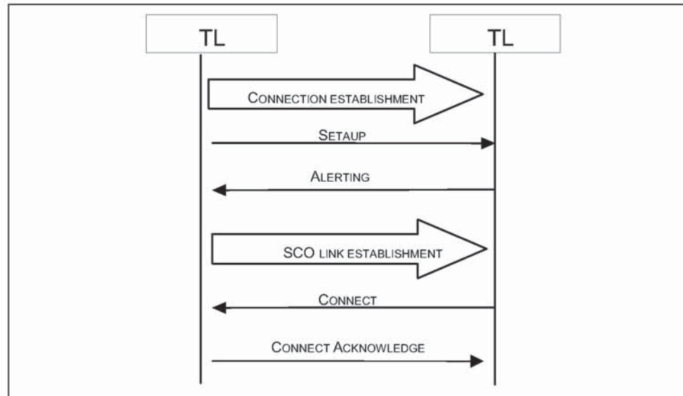
Figure 10.1: Call establishment
