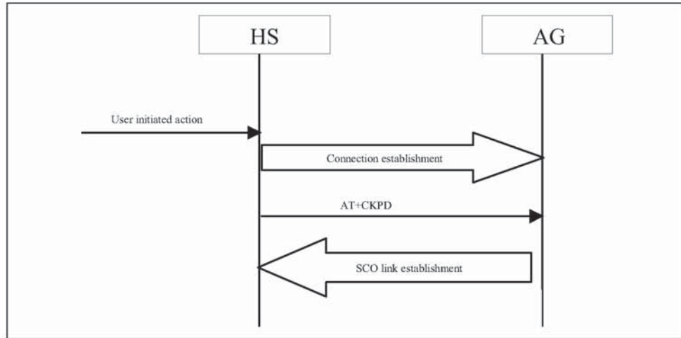
Figure 4.2: Outgoing audio connection establishment
