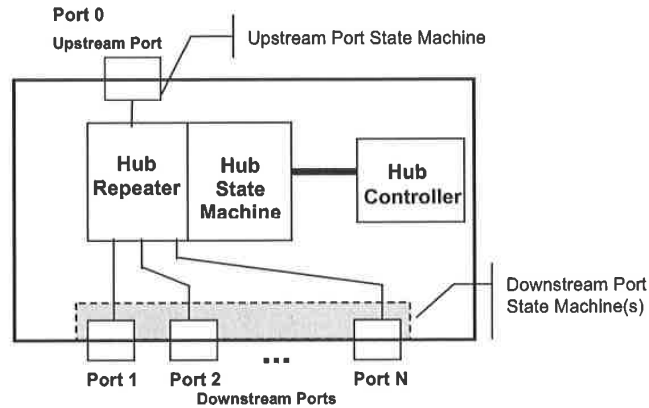
Figure 11-1. Hub Architecture
