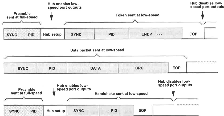
Figure 8-19. Low-speed Transaction
