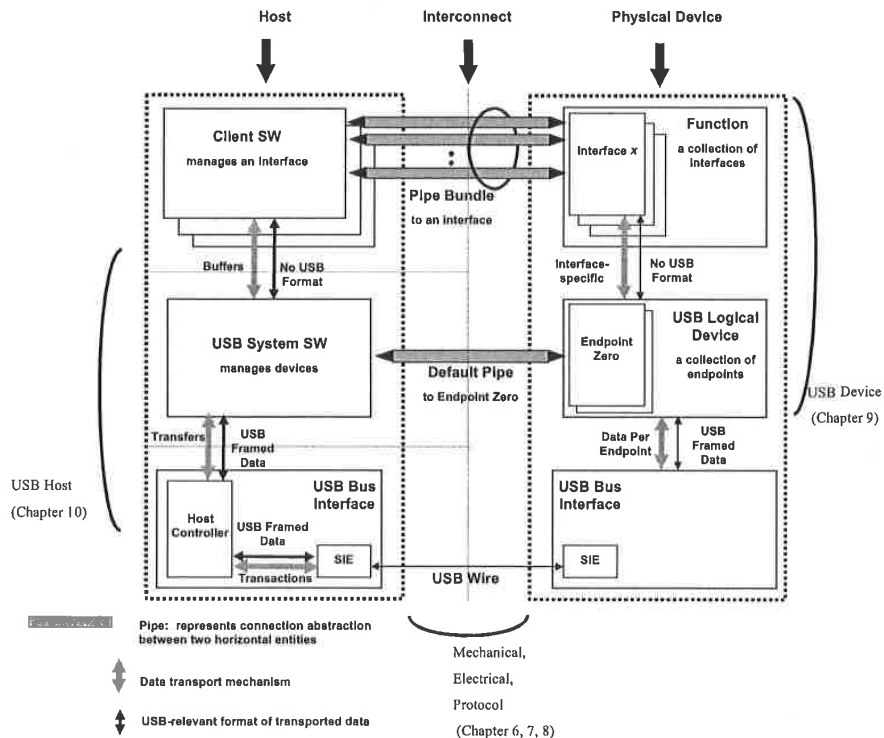
Figure 5-8. USB Host/Device Detailed View
