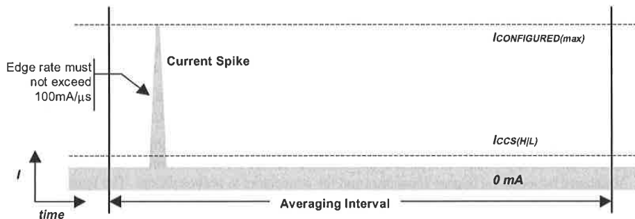
Figure 7-38. Typical Suspend Current Averaging Profile
