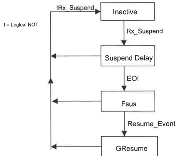
Figure 11-5. Internal Port State Machine
