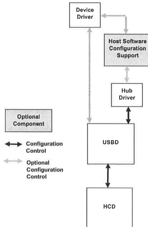
Figure 10-4. Configuration Interactions
