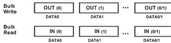
Figure 8-10. Bulk Reads and Writes
