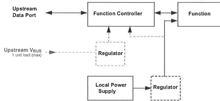
Figure 7-36. Self-powered Function
