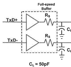
Figure 7-7. Full-speed Load
