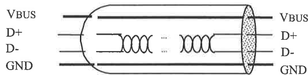
Figure 4-2. USB Cable
