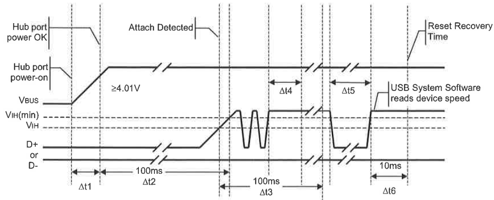
Figure 7-19. Power-on and Connection Events Timing
