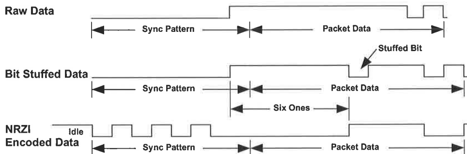
Figure 7-22. Bit Stuffing
