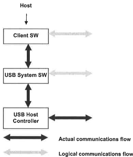
Figure 5-3. Host Composition
