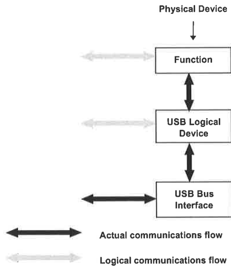
Figure 5-4. Physical Device Composition
