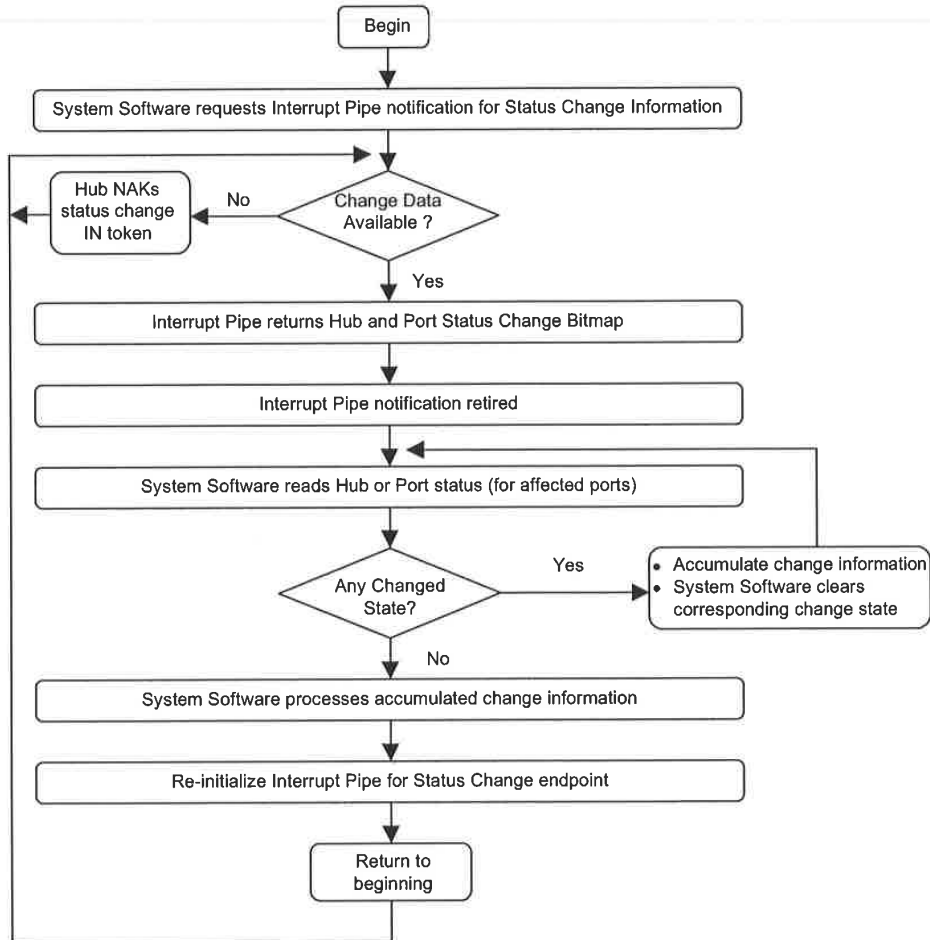
Figure 11-13. Port Status Handling Method
