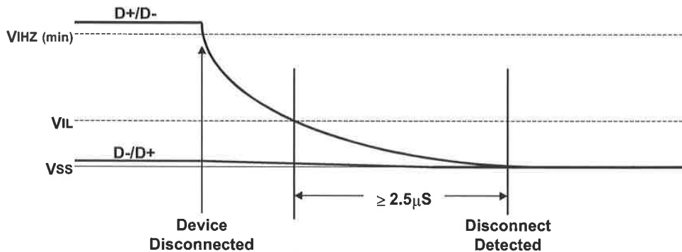
Figure 7-15. Disconnect Detection
