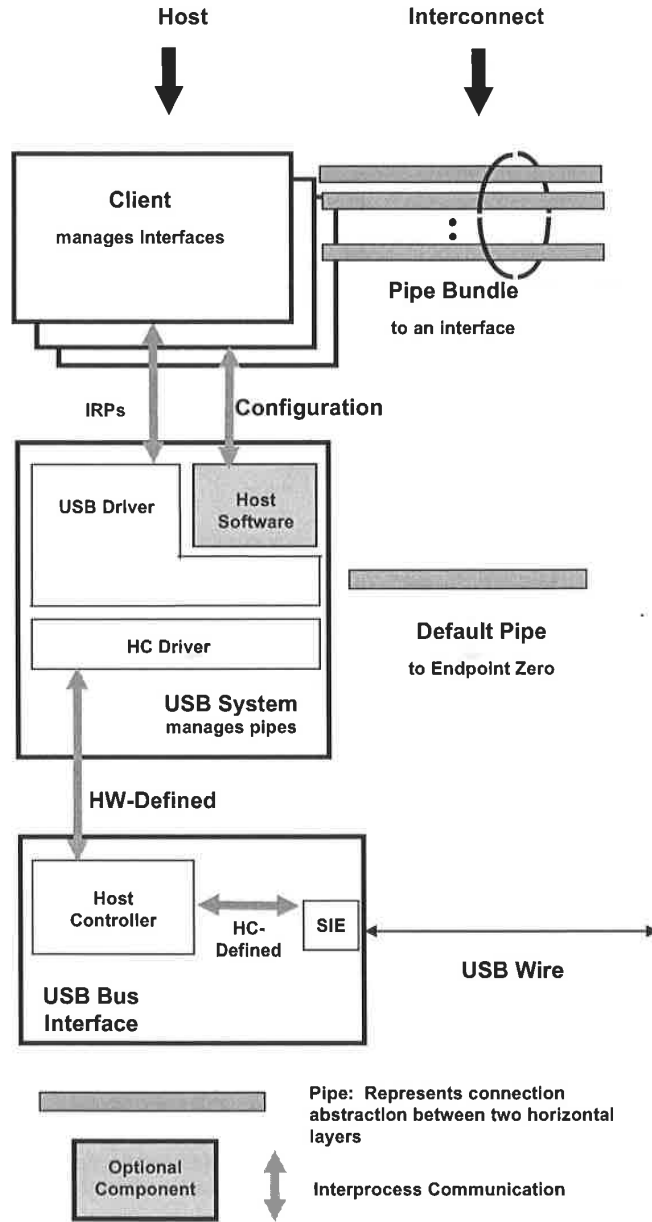
Figure 10-2. Host Communications
