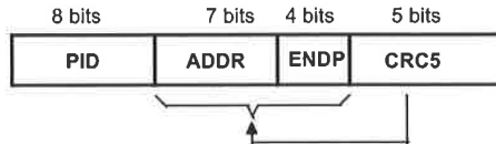
Figure 8-5. Token Format
