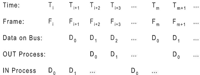
Figure 5-16. Data Prebuffering
