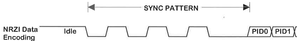
Figure 7-25. Sync Pattern
