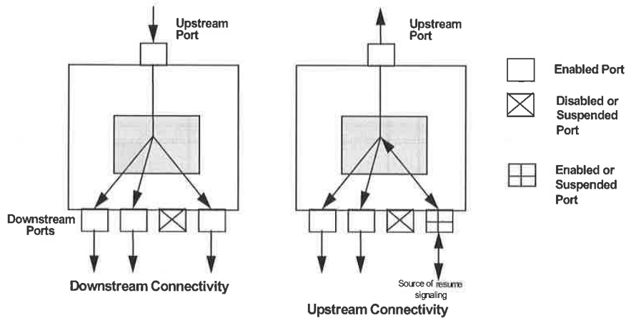
Figure 11-3. Resume Connectivity
