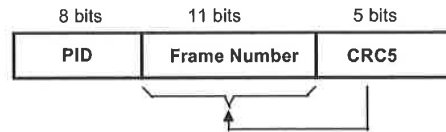
Figure 8-6. SOF Packet
