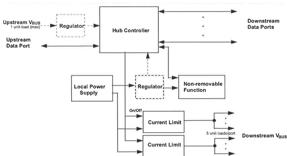
Figure 7-33. Compound Self-powered Hub
