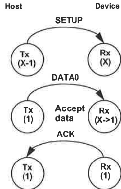
Figure 8-15. SETUP Initialization
