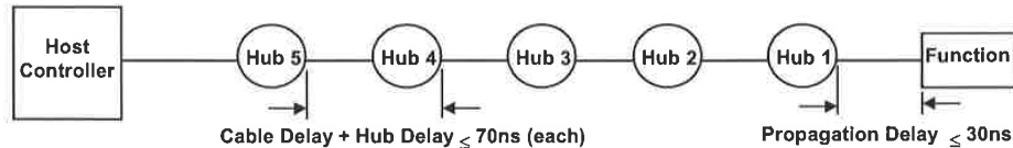
Figure 7-31. Worst-case End to End Signal Delay Model
