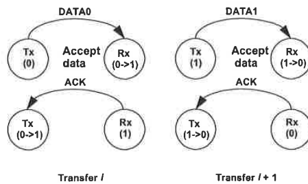
Figure 8-16. Consecutive Transactions
