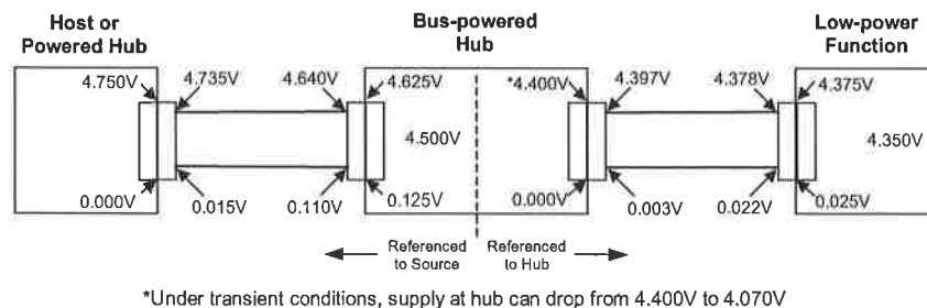
Figure 7-37. Worst-case Voltage Drop Topology (Steady State)
