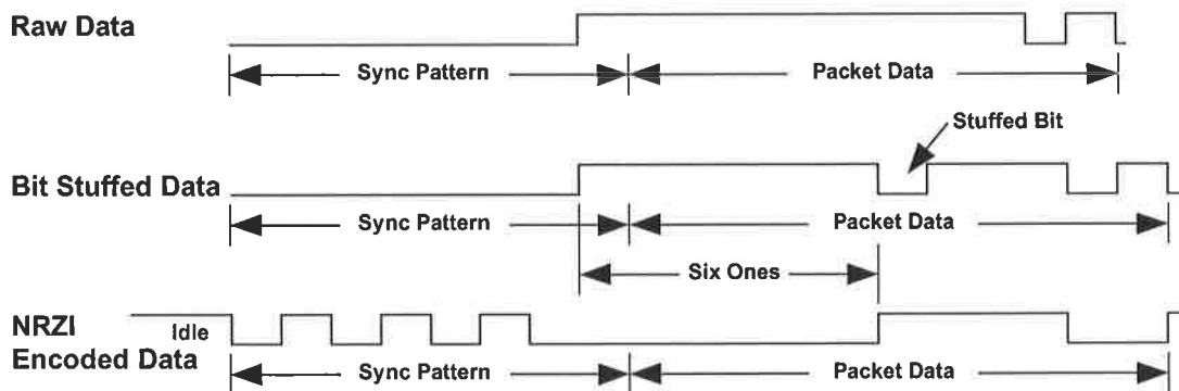
Figure 7-22. Bit Stuffing
