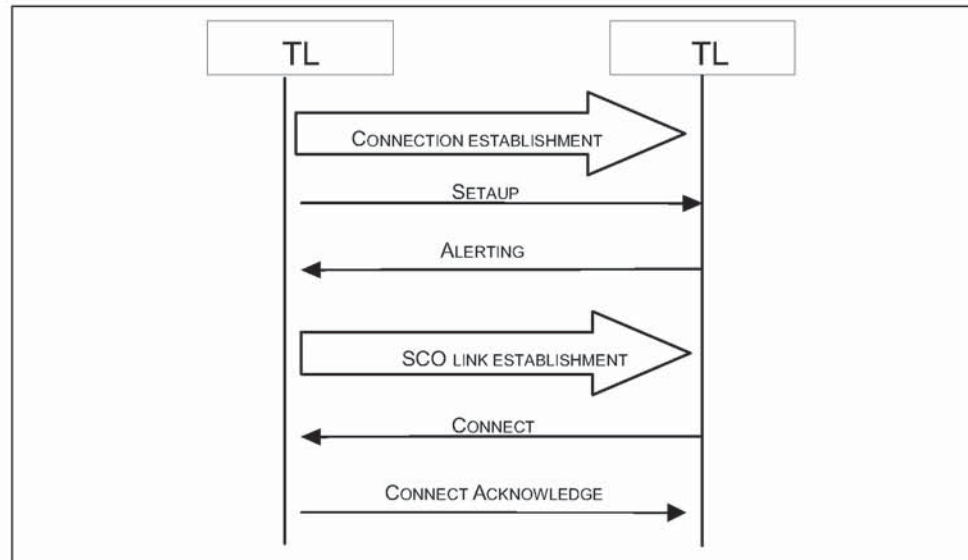
Figure 10.1: Call establishment
