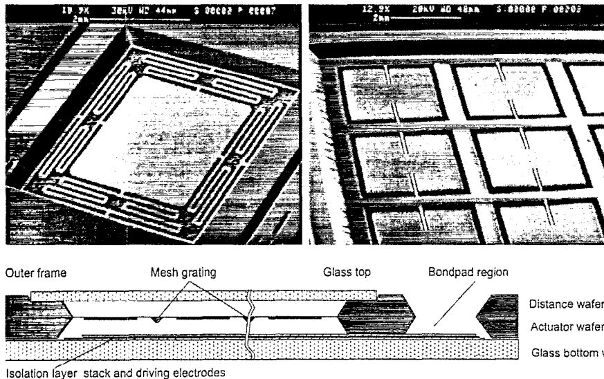
Fig. 2. SEM photograph of the back of a two-directional mirror and of a mirror array in bulk micromechanics and cross-sectional schematic view.
