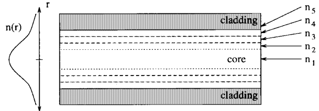
Fig. 6. Graded-index fiber.
