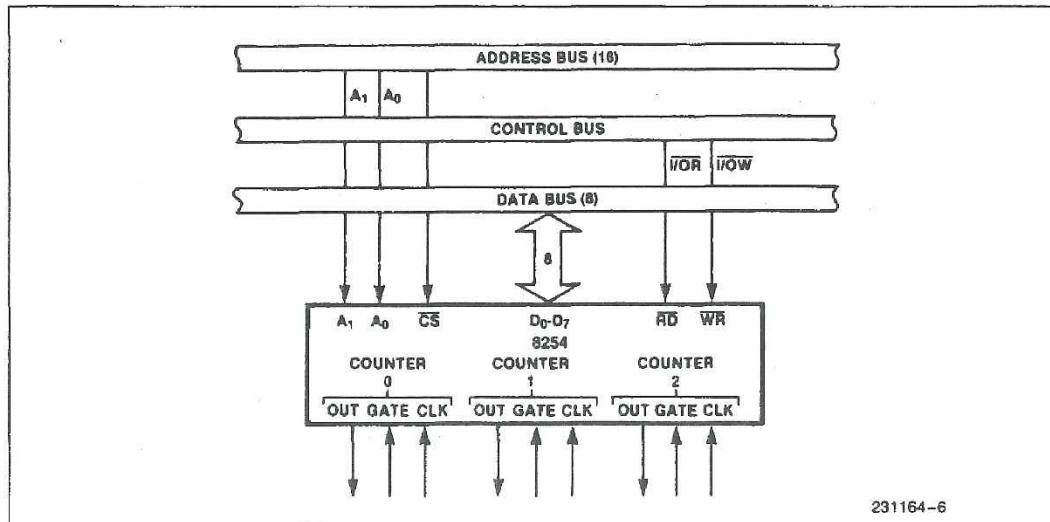
Figure 6. 8254 System Interface
