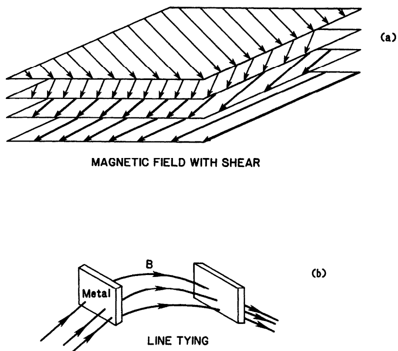
FIGURE 29. Two methods to stabilize interchange modes: a) magnetic shear, and b) line tying.
