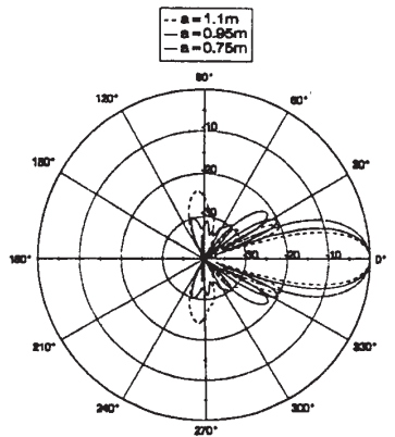
Figure 11: Antenna patterns versus array radius.
