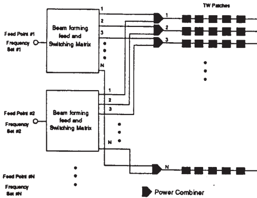
Figure 6: Scanning array with multiple beams.
