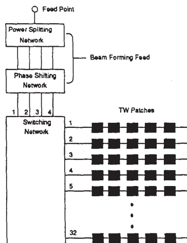
Figure 5: Scanning array system diagram.
