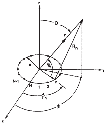
Figure 7: Circular array geometry.
