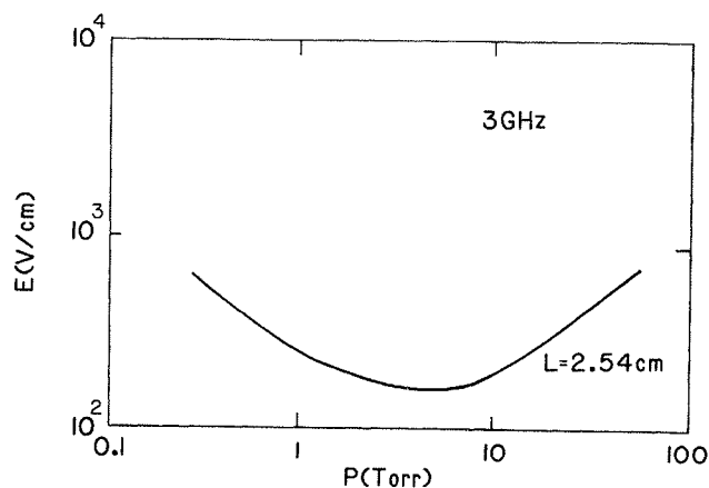
FIGURE 35. Rf Paschen curve for hydrogen in a vessel of 2.54 cm characteristic size (adapted from Ref. 3).
