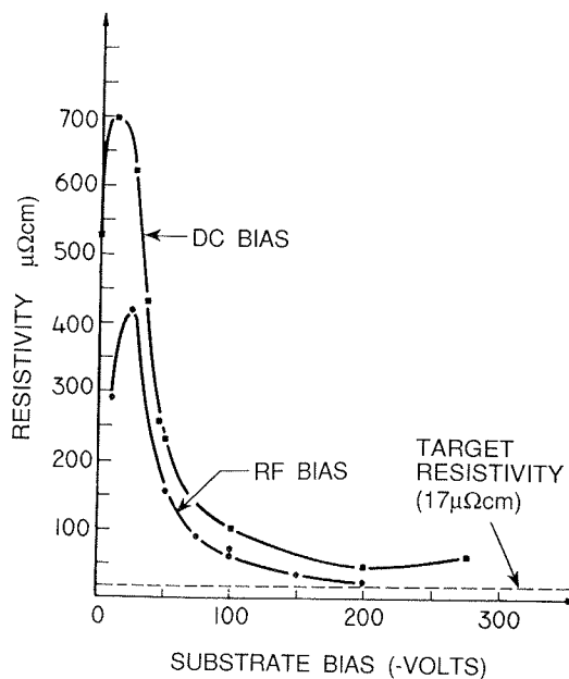
Figure 3-24. Resistivity of Ta films vs. substrate bias voltage; dc bias (3000 Å thick). (From Ref. 27). RF bias (1600 Å thick). (From Ref. 28).
