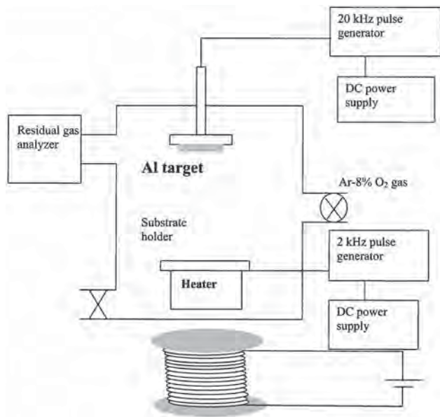
FIG. 1. Schematic diagram of the deposition chamber.
