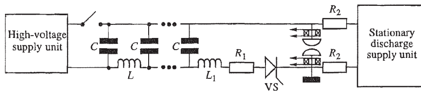
Fig. 2. Discharge supply unit.
