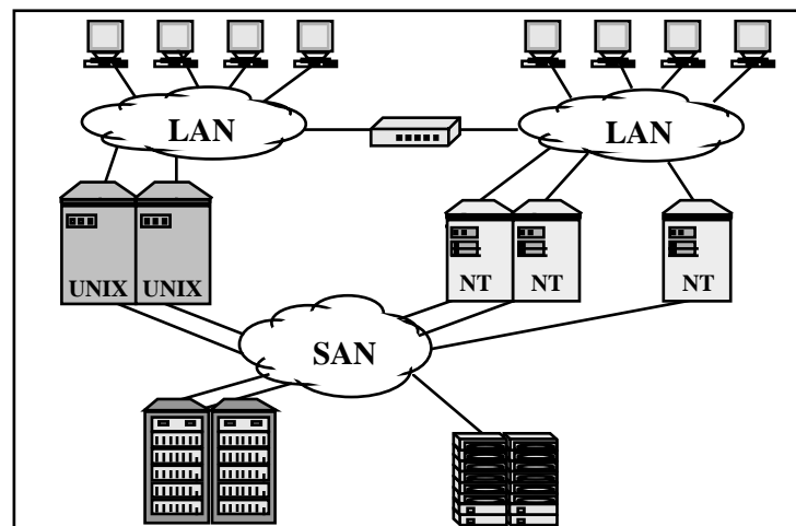
Figure 3. Server-Independent Storage
