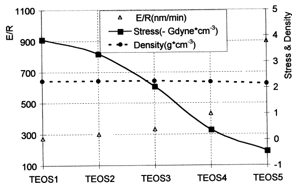
Fig. 2. Effects of TEOS/N 2 O gas flow ratio on film stress, NH 4 F-buffered HF chemical wet etch rate and film density of oxides.
