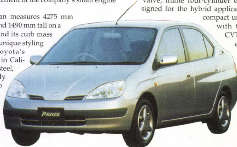
Toyota Prius is a compact four-seat sedan, measuring 4275 mm long, 1695 mm wide, and 1490 mm tall on a 2500-mm wheelbase.
