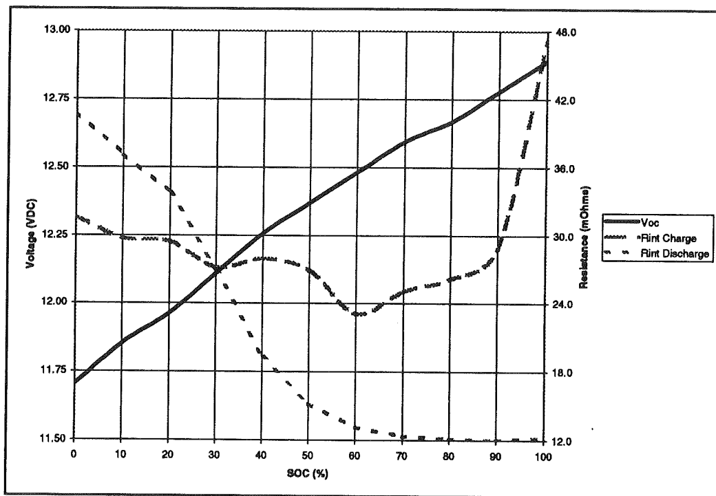
Figure 7. Battery Module Internal Resistance and Open-Circuit Voltage
