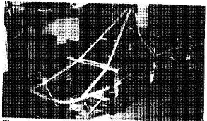
Figure 2: Formula Lightning Chassis
