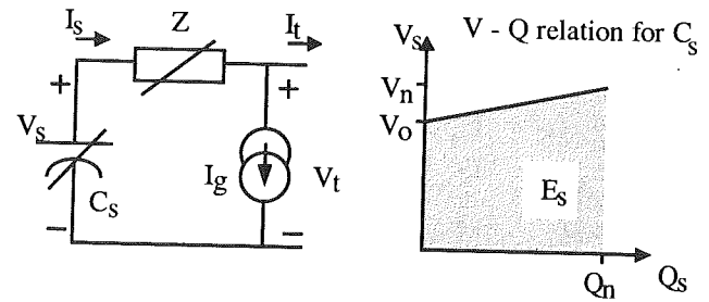
Figure 1: Electrical equivalent circuit model used for battery state controllers. The model obeys conservation of charge and energy, and includes a gassing circuit. The plot of V_s vs. Q_s shows the open circuit voltage relation, while the shaded area represents stored energy.
