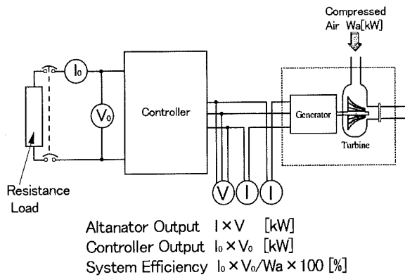
Fig.5 Schematic of Component Test
