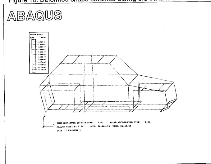
Figure 11. Maximum stresses obtained during the flexural calculation.
