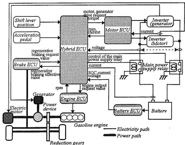
Fig.7 ECU Schematic
