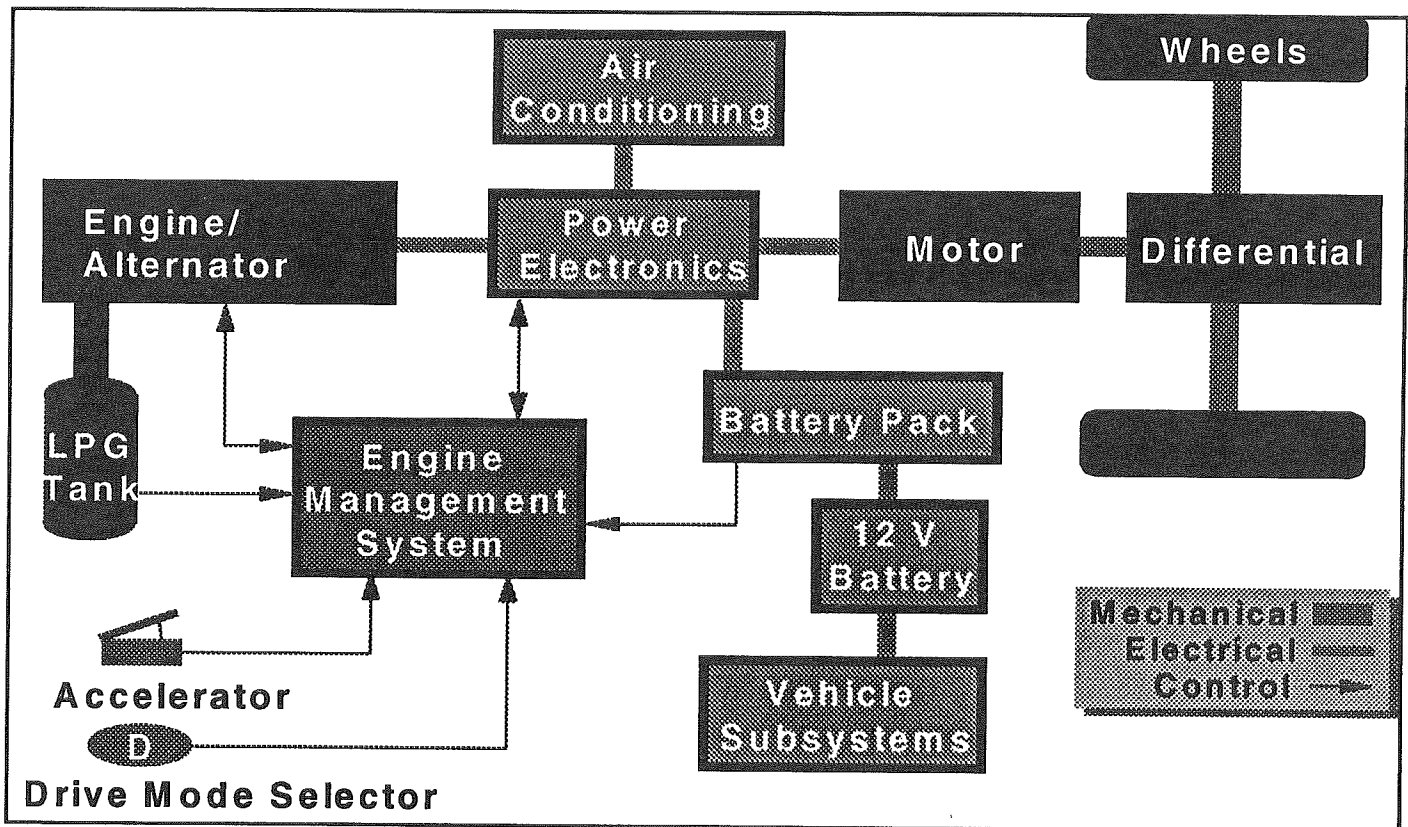
Figure 3. Virginia Tech FutureCar System Schematic
