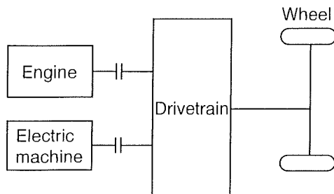
Fig. 1 Hybrid drivetrain
