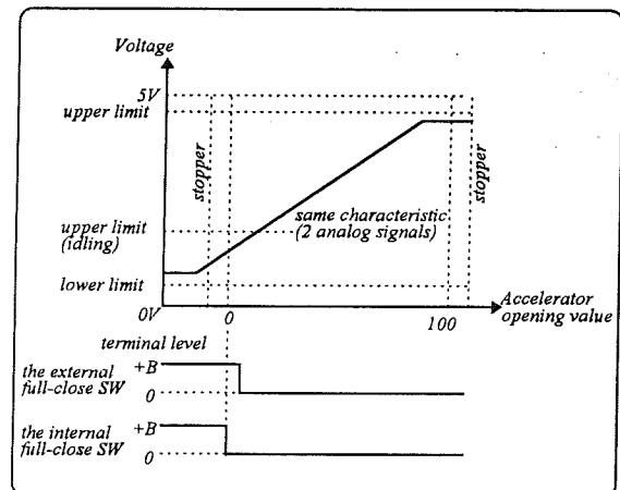
Fig.13 Accelerator Sensor 2
