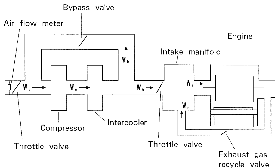
Fig. 3 Intake system
