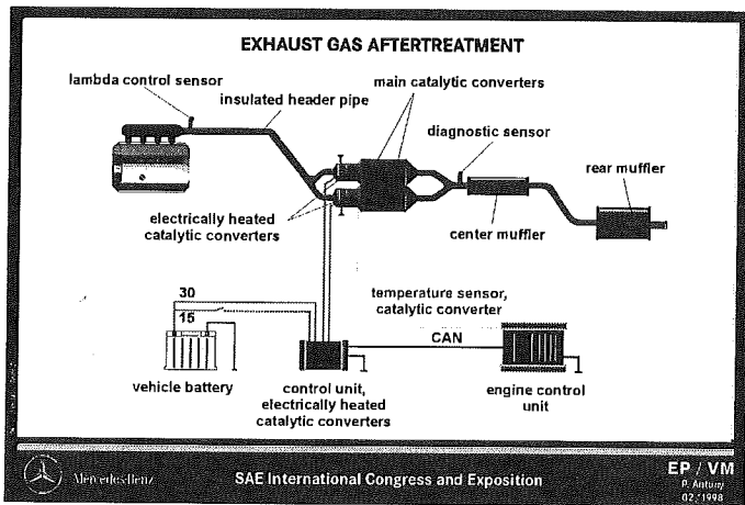
Figure 7. Exhaust gas aftertreatment system
