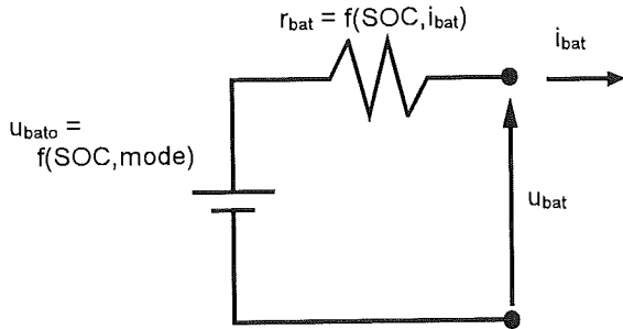
Fig. 3: Battery Model
