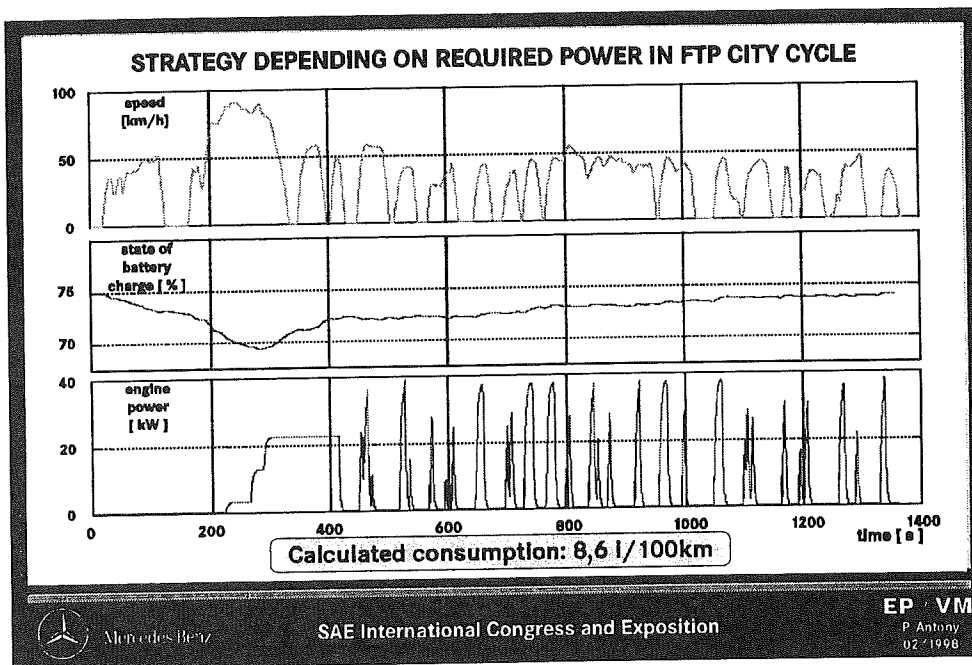
Figure 16. Power-dependent strategy in the FTP75 test
