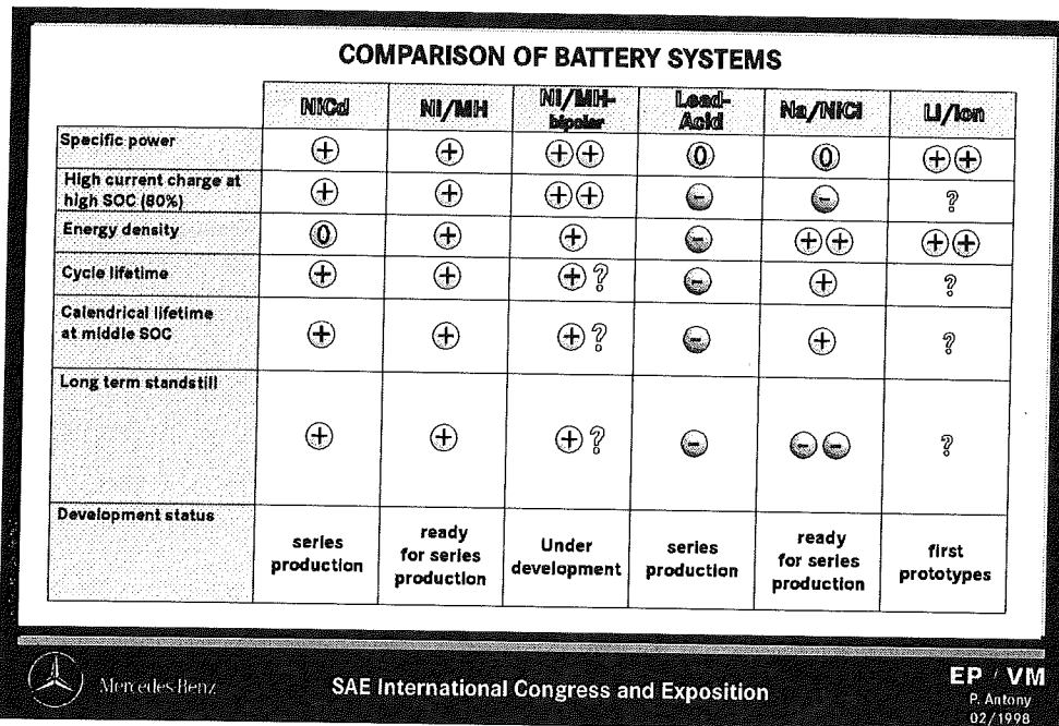
Figure 12. Current battery systems
