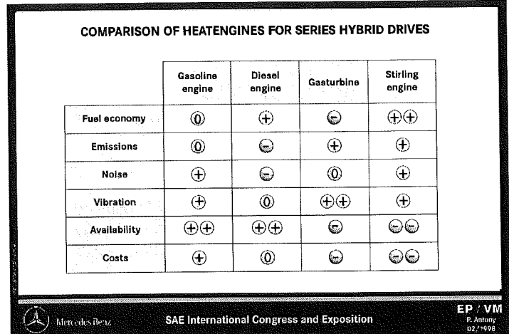
Figure 6. Comparison of heat engines for series hybrids
