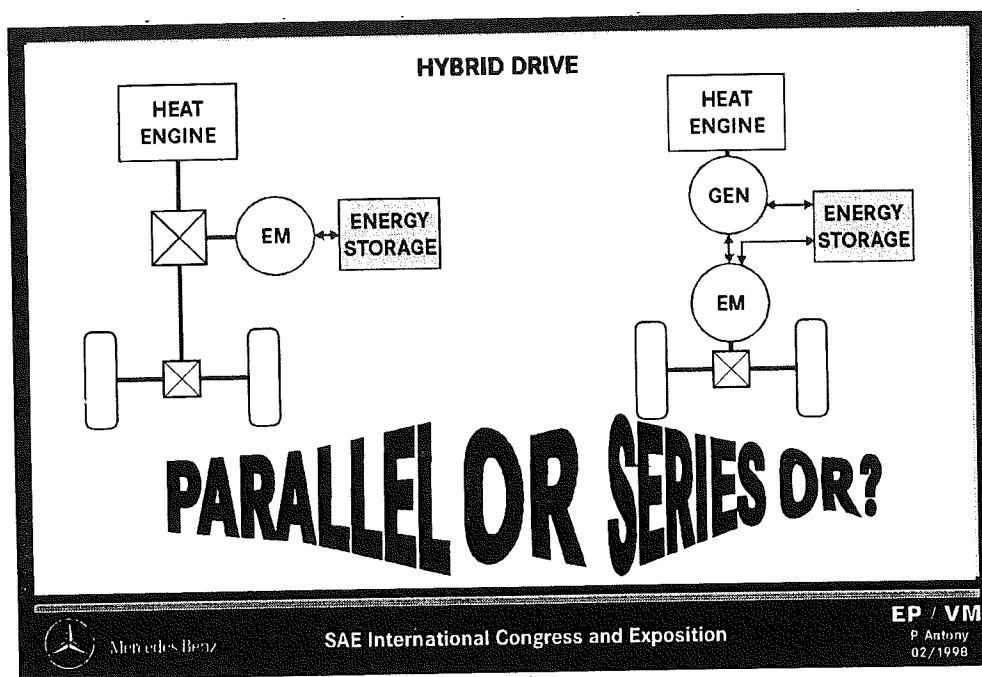
Figure 1. Parallel and series hybrid concept
