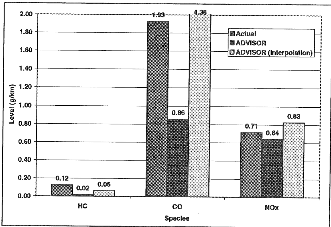
Figure 17. SOC-Corrected FUDS Emissions Comparison
