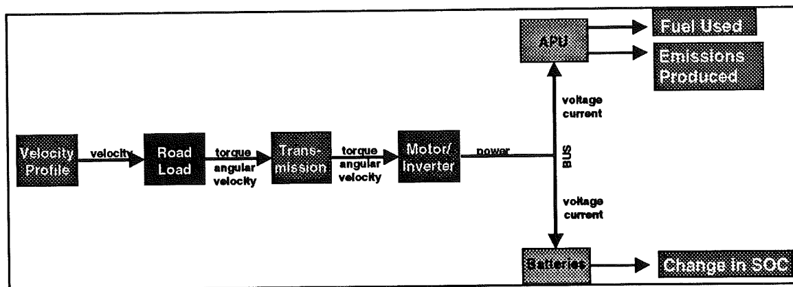
Figure 2. ADVISOR Series HEV Data Flow
