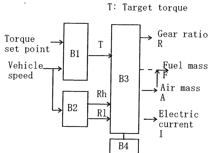
Fig. 2 Control system
