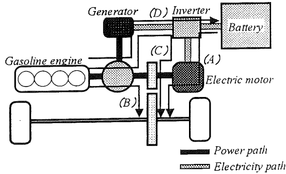
Fig.2 Operating Conditions
