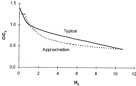
Fig. 5: Battery Capacity Versus Discharge Current
