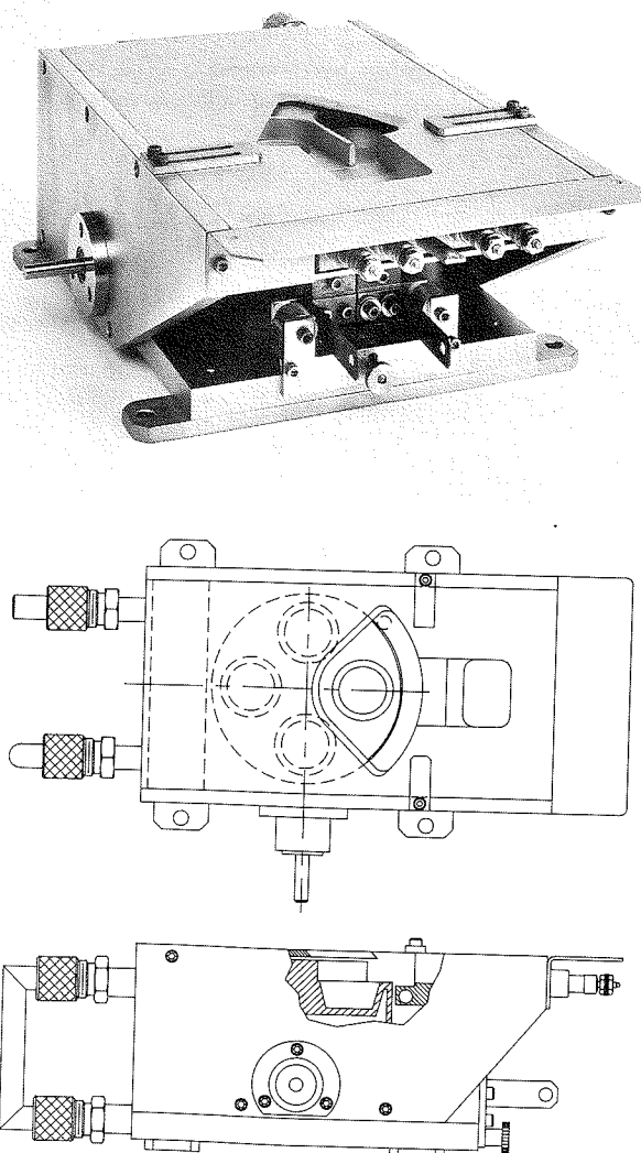
Figure 3-12. Multihearth electron beam evaporation unit with accompanying schematics. (Courtesy of Temescal unit of Edwards High Vacuum International, a division of the BOC Group, Inc.).
