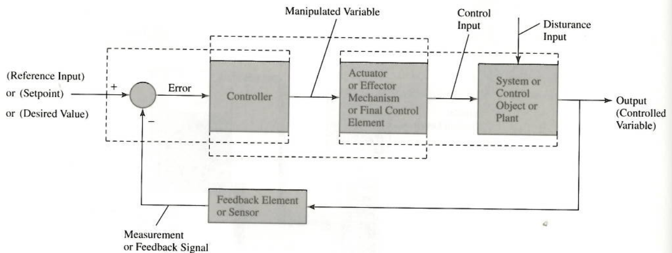
Figure 1.6 Typical Feedback Control Structure
