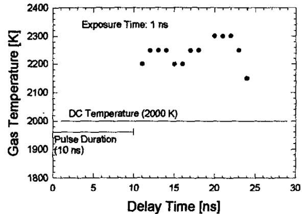
Figure 4. Temporal Development of the gas temperature in the center of a MCSG discharge operated DC with superimposed pulse. Electrode distance: 2 mm, I_{MCSG DC} = 10 mA.
