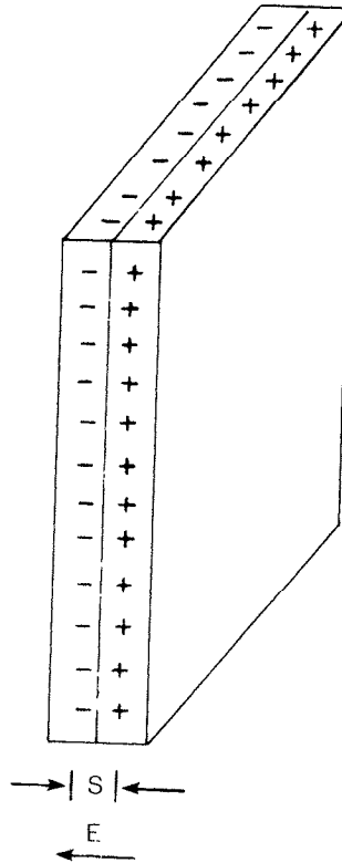
FIGURE 15. Collection of charged particles in a slab. The positive particles were displaced from the negative. A strong electric field results, which will force the two sets of particles back toward each other.
