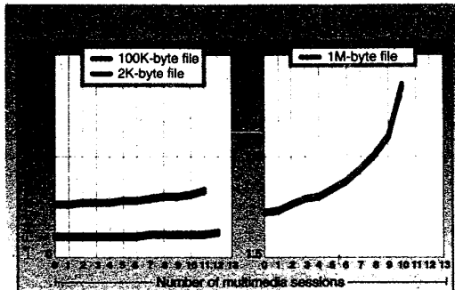
Figures show the effect of multimedia sessions on server-to-client file-transfer times. The IBM bitnet Token-Ring test network supported 13 Personal System/2 clients and 3 OS/2 servers — 2 for multimedia traffic and 1 for data — outfitted with new Busmaster Token-Ring adapters.
