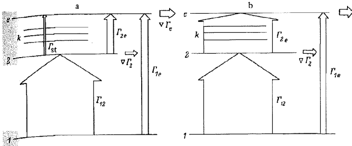
FIG. 1. Diagram showing the relative sizes of the electron fluxes in terms of the atomic energy levels for the slow (a) and fast (b) stages. The width of the arrows indicates the magnitude of the electron flux. The horizontal arrows give the diffusion fluxes of electrons and excited atoms reaching the walls of the discharge tube.
