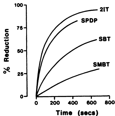
Fig. 5. Rates of reduction by DTT of IgG derivatized with various coupling agents. Bovine IgG was reacted with SMBT, SBT, 2IT, or SPDP and the derivatives were reduced with DTT and treated with Ellman's reagent to form antibody derivatives in which the same activated disulfide group was present in all. The derivatives were then treated with 0.03 mM DTT at pH 7.4 and 25°C. The rate of release of the 3-carboxylato-4-nitrothio phenolate group was followed spectrophotometrically at 412 nm. The A_{412} at various times after adding DTT is expressed as a percentage of the A_{412} after complete reduction with 5 mM DTT.
