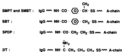
Fig. 4. Linkages formed by the different coupling agents.
