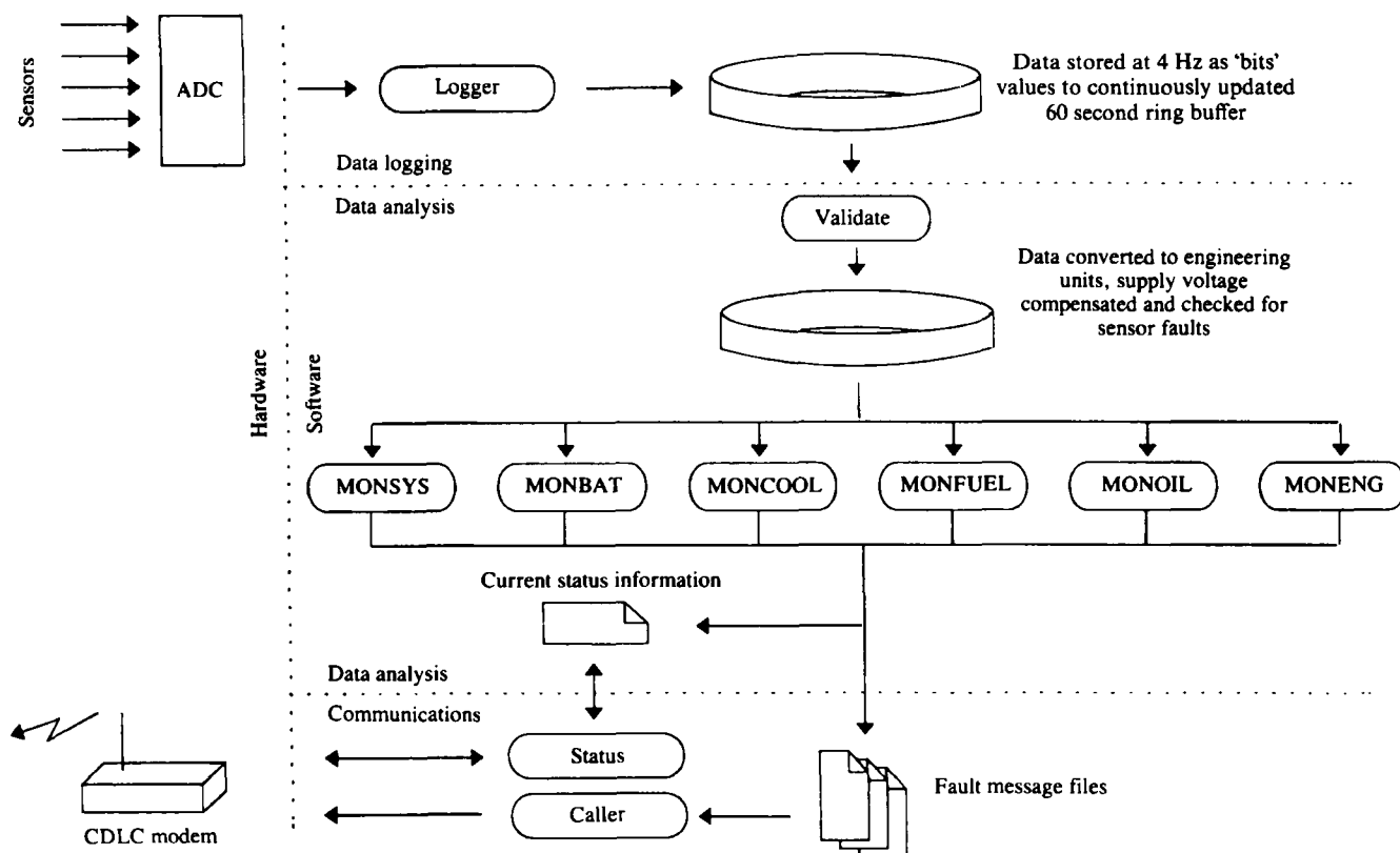
Fig. 4 Structure of DEMON SMR47 software
