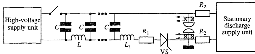
Fig. 2. Discharge supply unit.
