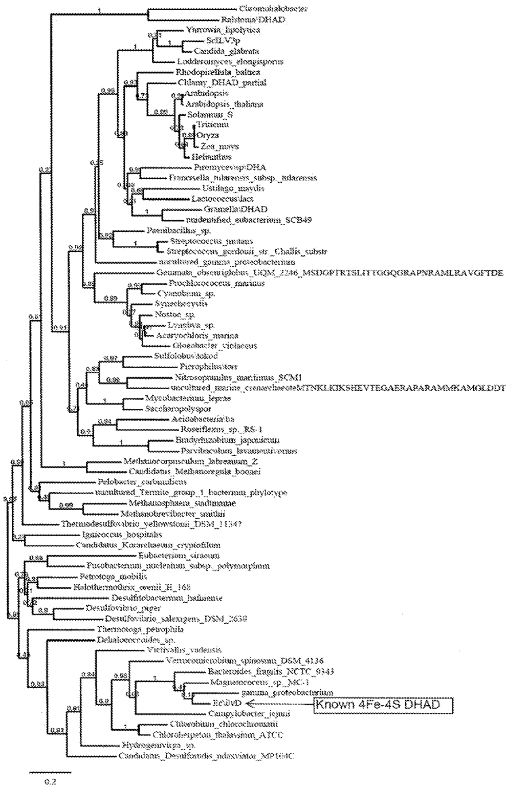
Figure 2. Phylogenetic tree of DHAD proteins. Numbers at nodes indicate bootstrap values. EcolivD is a known 4Fe-4S DHAD enzyme from Escherichia coli .
