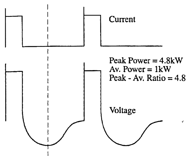
Fig. 8. Peak power.
