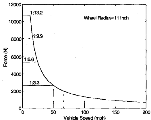
Fig. 1. Torque-speed diagram of an electrical motor in terms of tractive force and vehicular speed with gear size as the parameter.
