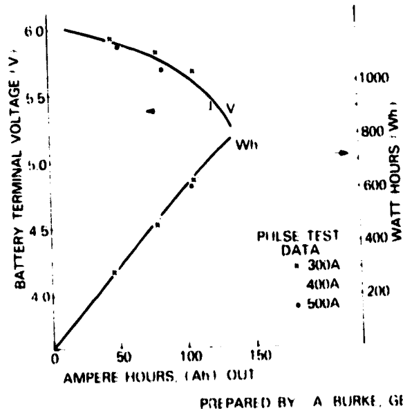
DISCHARGE CHARACTERISTIC OF THE ESB EV 105 AT 60A
