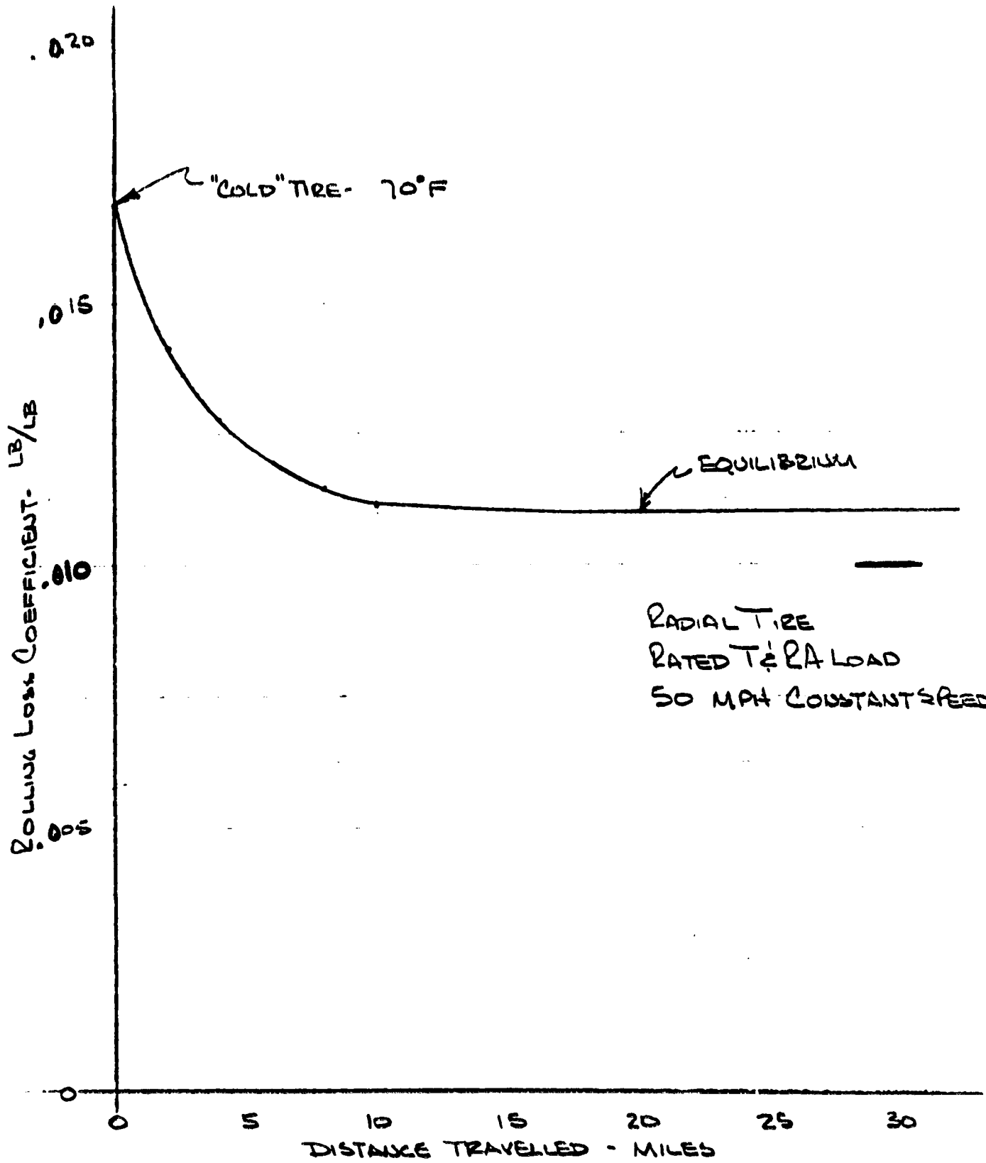
INFLUENCE OF DISTANCE TRAVELLED ON TIRE DEGR.
