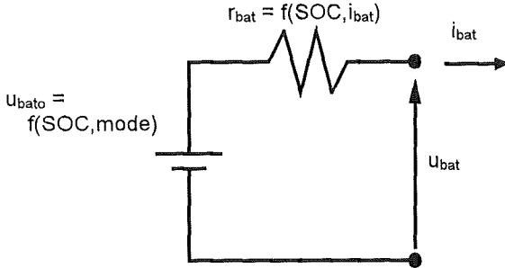
Fig. 3: Battery Model
