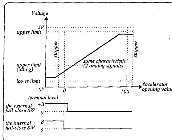
Fig.13 Accelerator Sensor 2
