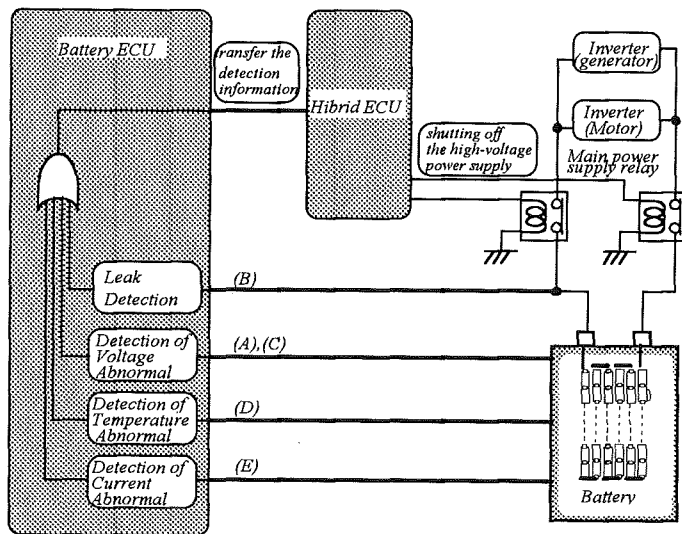
Fig.16 Fail-Safe
