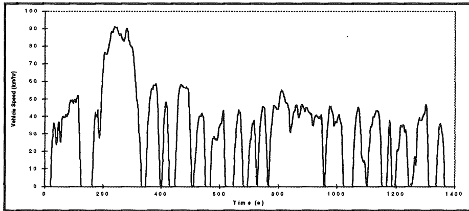
Figure 9. FHDS Driving Trace
