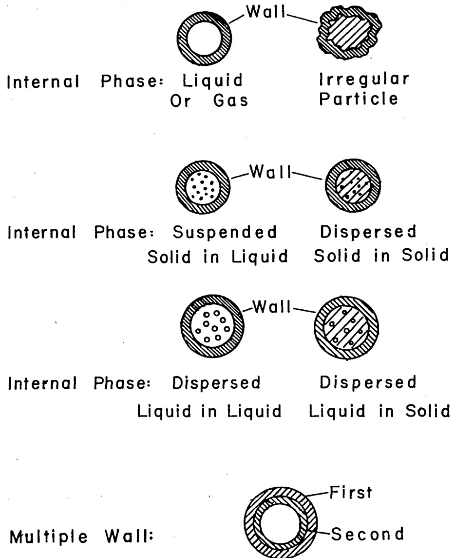
FIGURE 1. Capsule Configuration.
