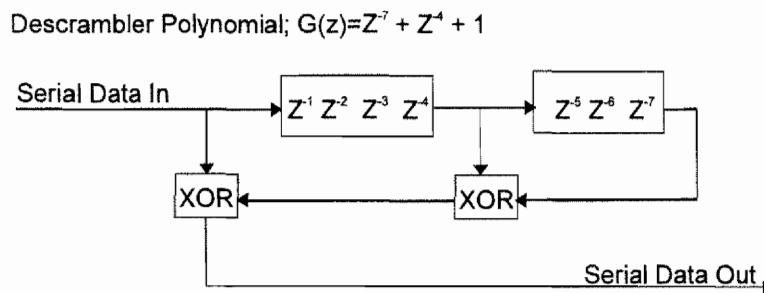
Figure 90—Data descrambler
