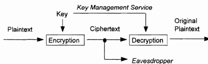
Figure 43—A confidential data channel
