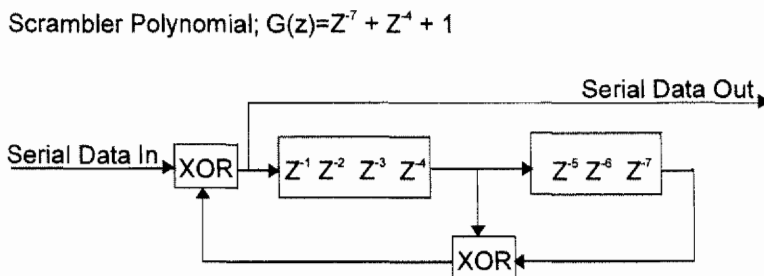
Figure 89—Data scrambler
