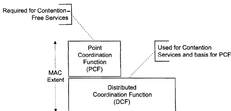
Figure 47—MAC architecture
