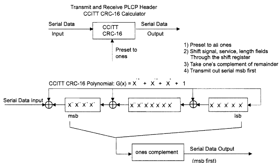
Figure 87—CCITT CRC-16 implementation
