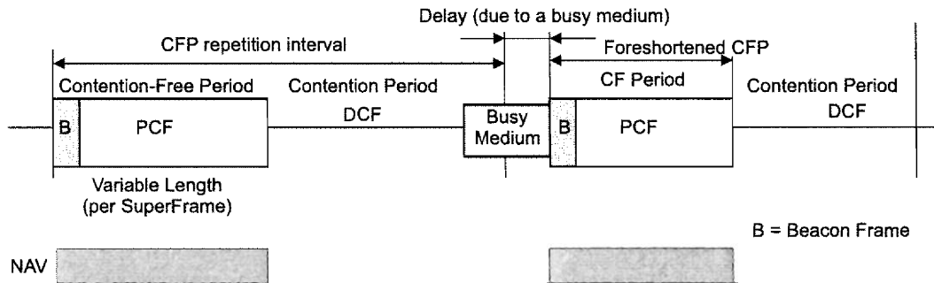
Figure 59—CFP/CP alternation
